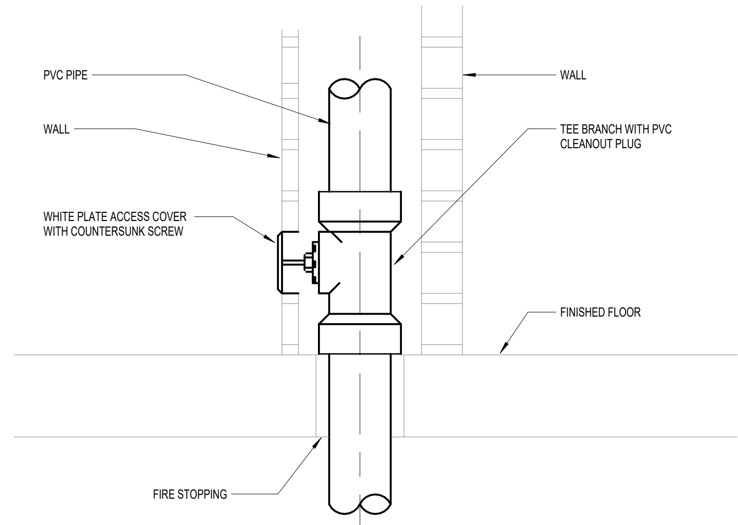
C1 WALL CLEANOUT NOT TO SCALE
