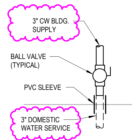
A2 DOMESTIC WATER METER DETAIL NOT TO SCALE
