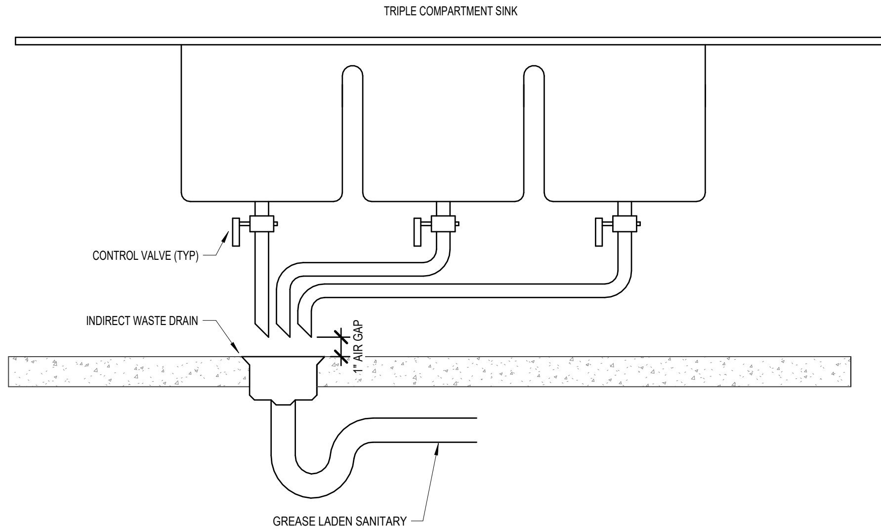
C3 TRIPLE SINK WITH INDIRECT DRAINAGE NOT TO SCALE
