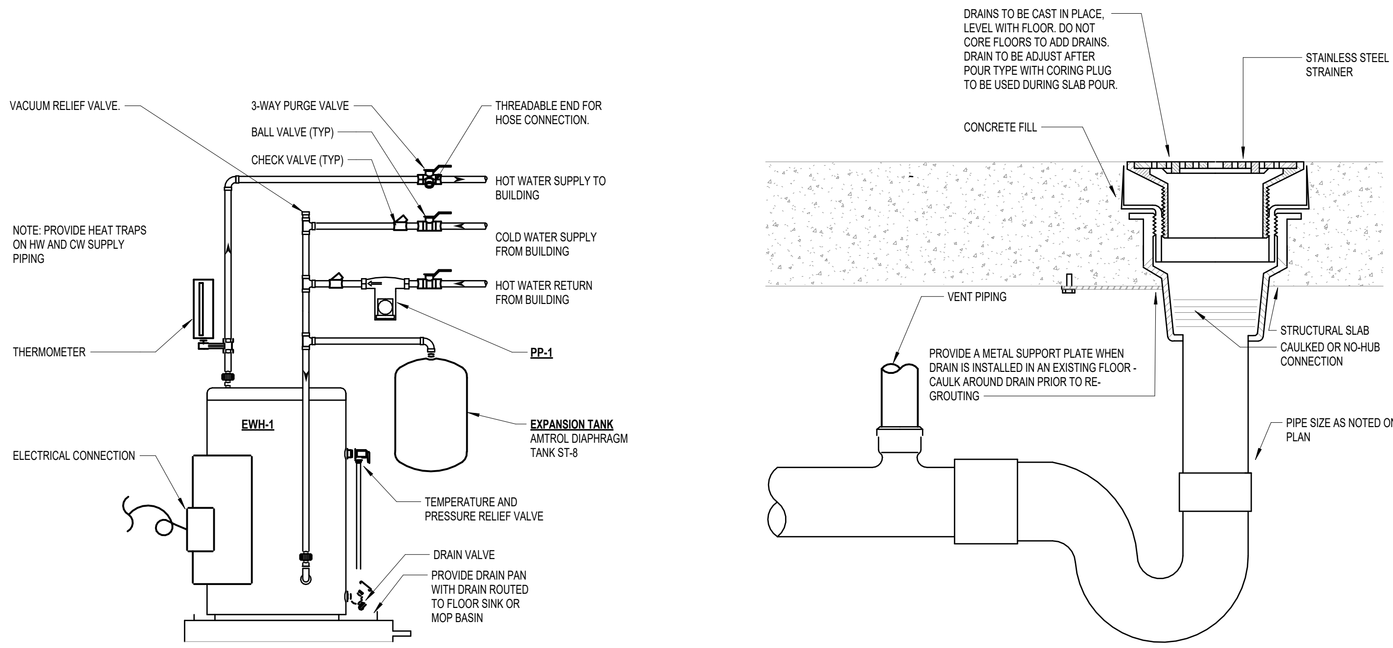
E4 WATER HEATER NOT TO SCALE
