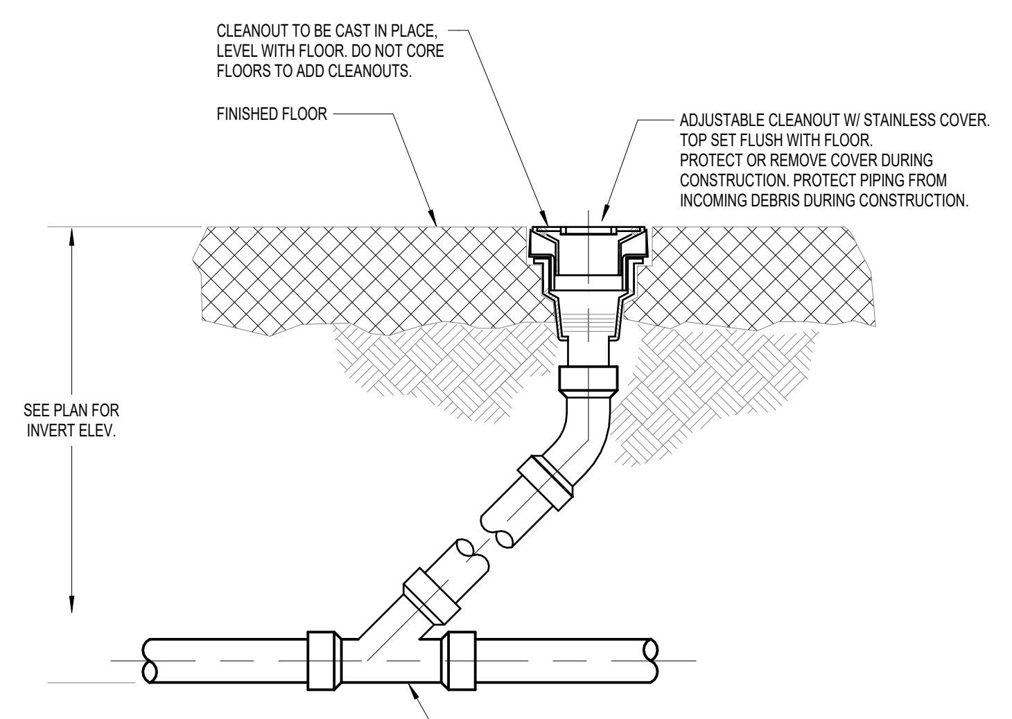
E1 CLEANOUT TO FINISHED FLOOR NOT TO SCALE
