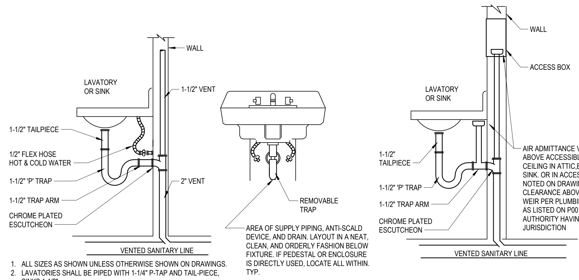
A1 TYPICAL SINK/LAVATORY DETAIL NOT TO SCALE
