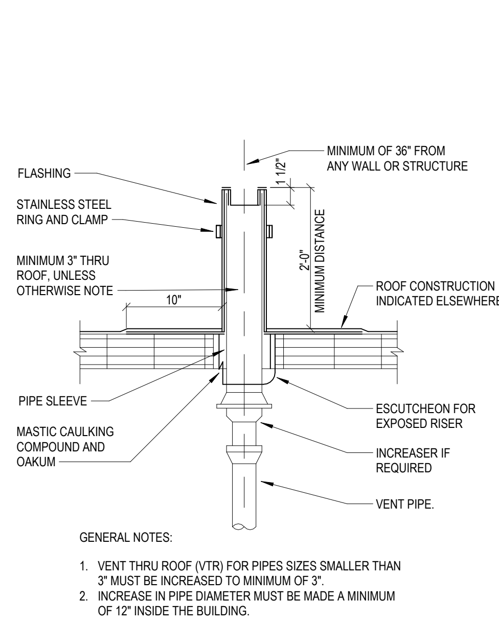
C4 PLUMBING VENT THROUGH ROOF DETAIL NOT TO SCALE
