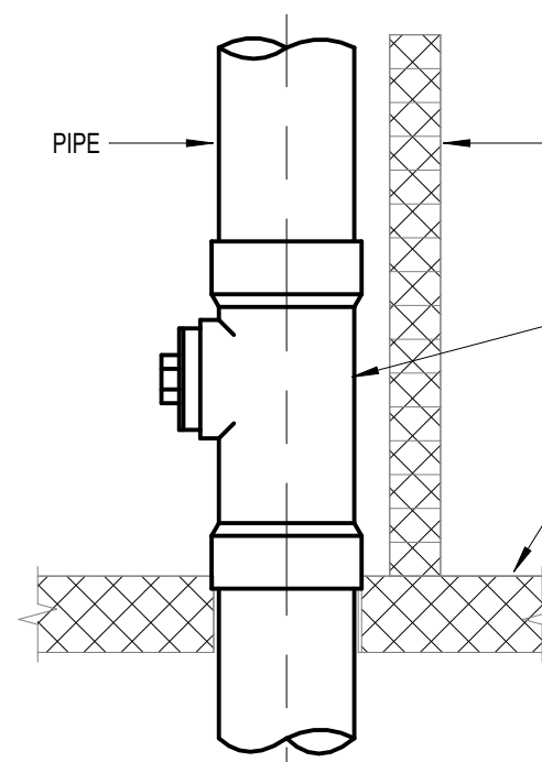
C2 RISER CLEANOUT NOT TO SCALE
