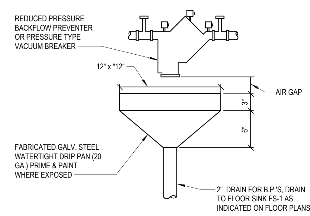
E2 BACKFLOW PREVENTER DRIP PAN DETAIL NOT TO SCALE
